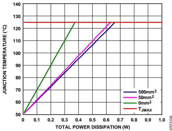
Figure 36. Junction Temperature vs. Total Power Dissipation, T_A = 50^\circ\text{C}
