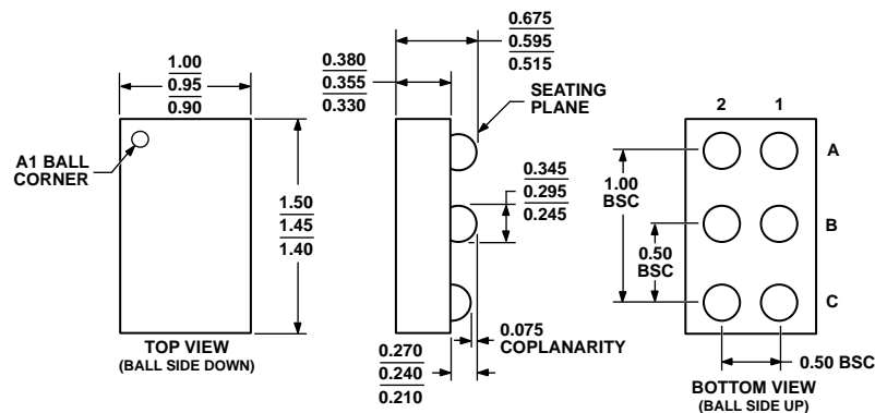
Figure 42. 6-Ball Wafer Level Chip Scale Package [WLCSP] (CB-6-2)
